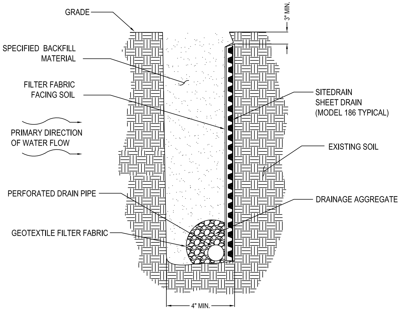
FOR CUT-OFF DRAIN > 3.5' DEEP
