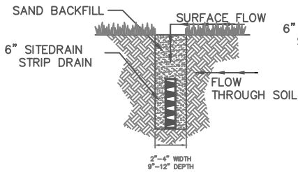
FIELD DRAIN DETAIL
