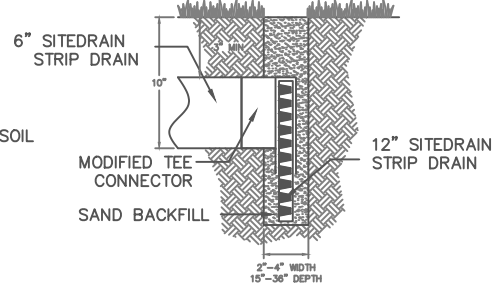
PERIMETER DRAIN DETAIL
