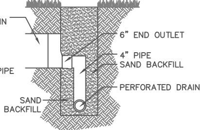
PERIMETER DRAIN DETAIL PIPE OPTION
