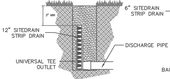
PERIMETER DRAIN DETAIL
