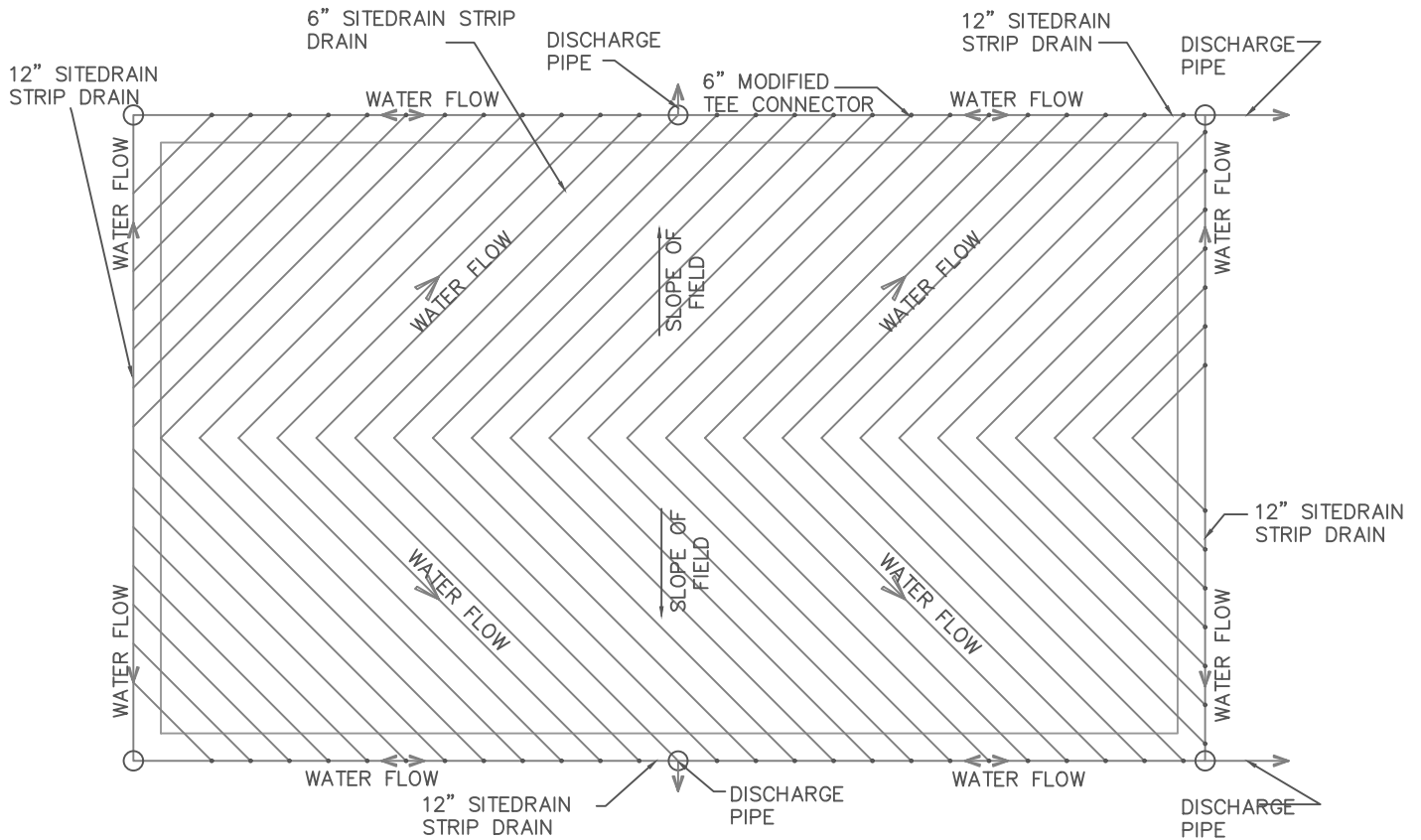
FIELD DRAIN DETAIL
