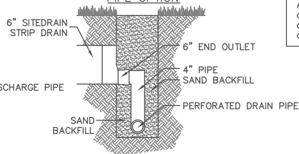
PERIMETER DRAIN DETAIL PIPE OPTION
