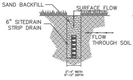
FIELD DRAIN DETAIL
