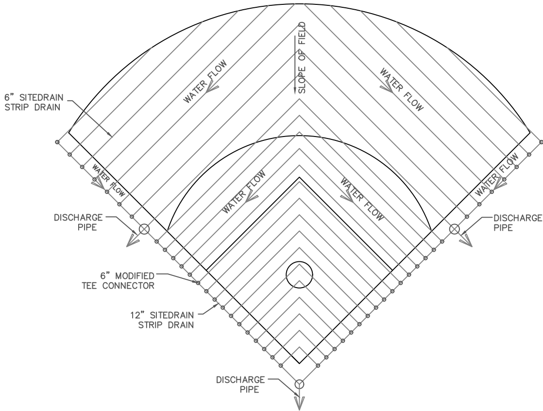
FIELD DRAIN DETAIL
