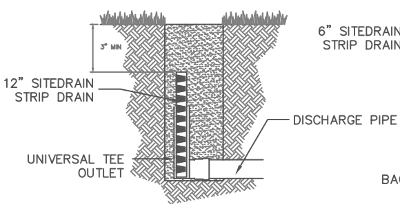
PERIMETER DRAIN DETAIL
